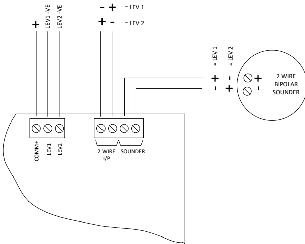
CONNECTION TO 2-WIRE BIPOLAR SOUNDER FOR DIFFERENT SOUNDS ON LEVEL 1 AND LEVEL 2
