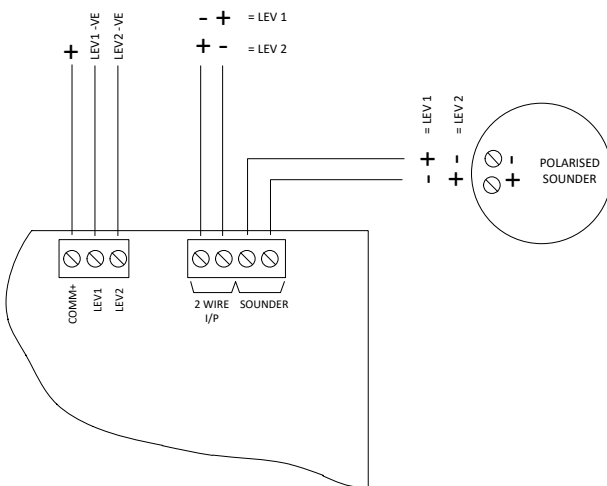
CONNECTION TO 2-WIRE POLARISED SOUNDER WHICH SOUNDS ON LEVEL 2 ONLY
